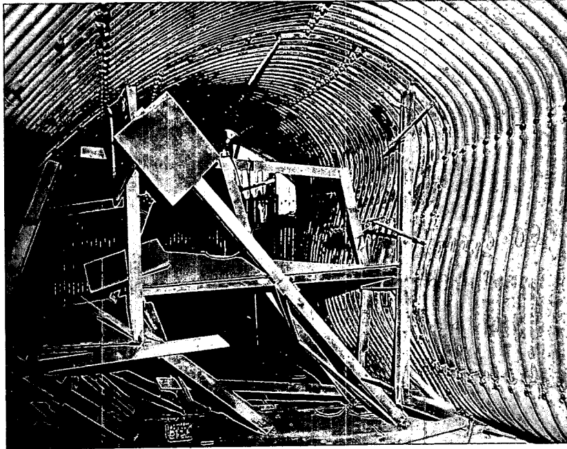
Fig. 5—Interior of building 3.6 after shot.
